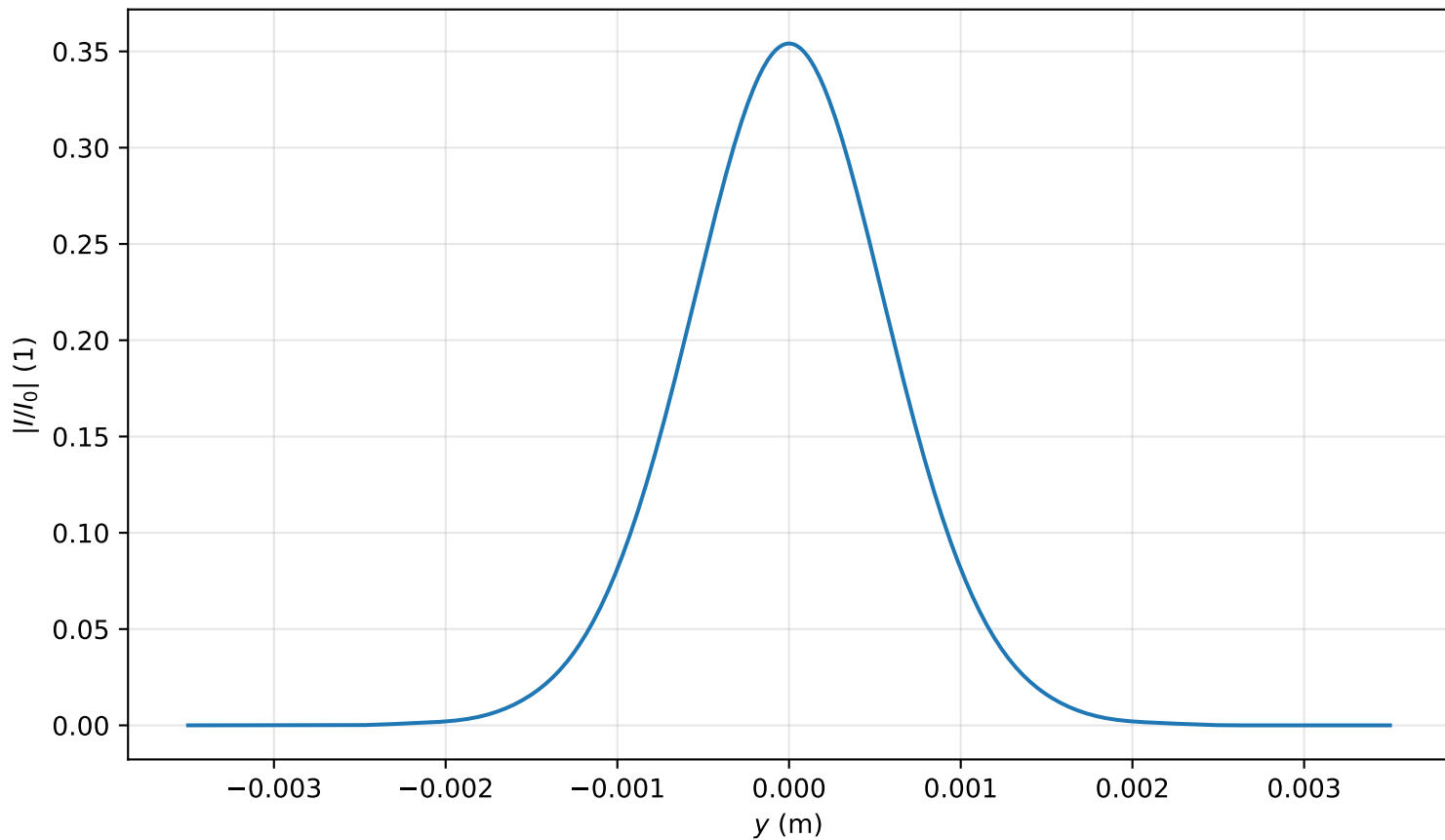
Intensity profile I(x=0, y, z=3.423)/I_0 , P_{in}=0.3P_{cr} , artificial time
